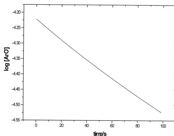
Fig. 2 Plot of log [ArO - ] vs. time for theoretical data calculated for the reaction between p -nitrophenoxide ion (0.00006 M) with methyl iodide (1 M) in acetonitrile containing water (0.04%) according to the mechanism illustrated in eqn. 4. The rate constants used were those reported for this reaction at 298 K ( k f = 0.00819 M -1 s -1 , k b = 0.00408 s -1 and k p = 0.0150 s -1 ). 2
